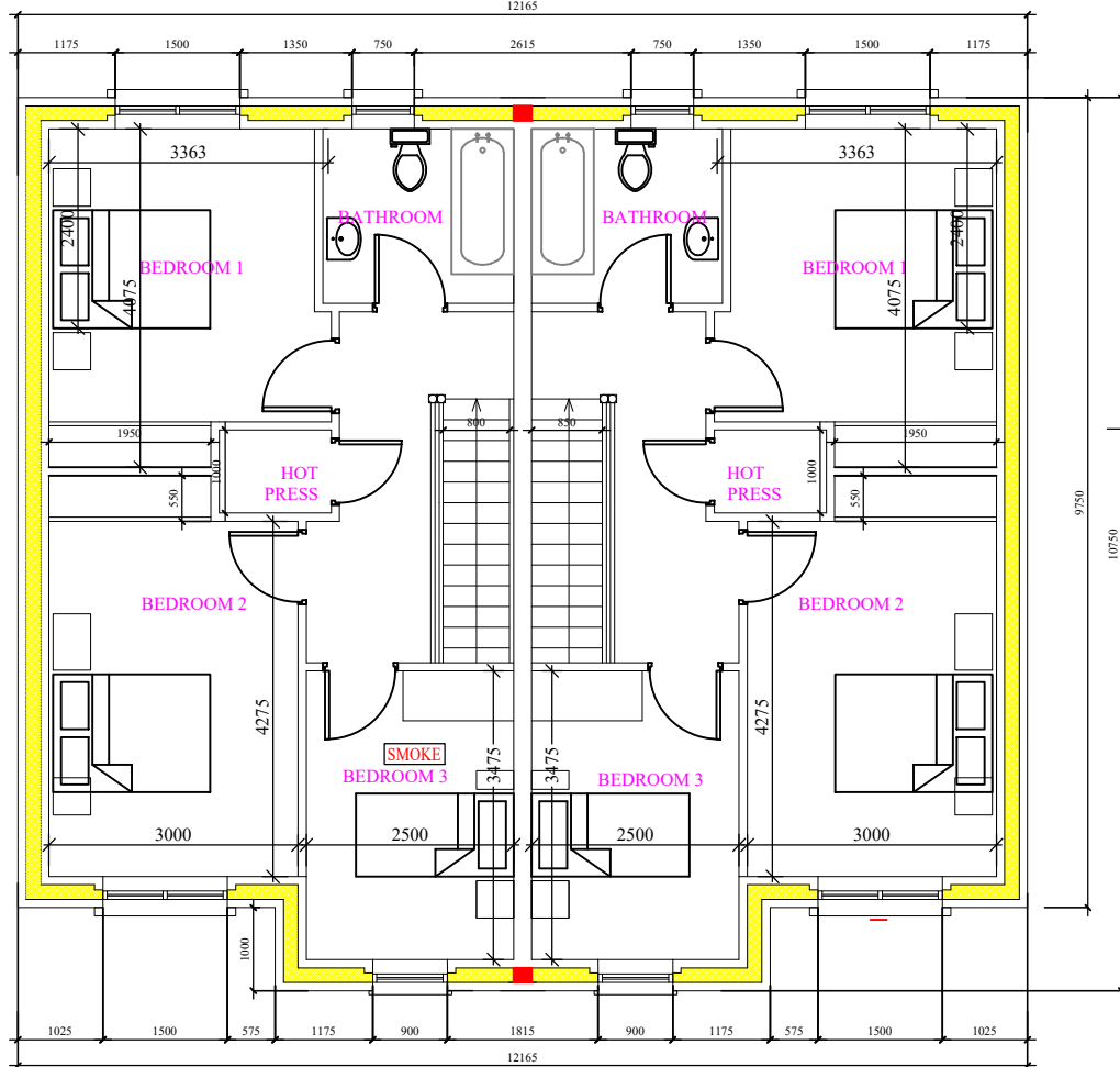
FIRST FLOOR PLAN UNIT AREA: 52.9sq.m
