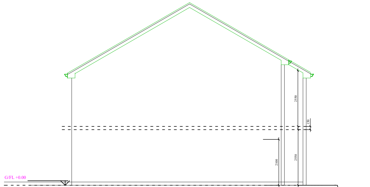
SIDE ELEVATION
